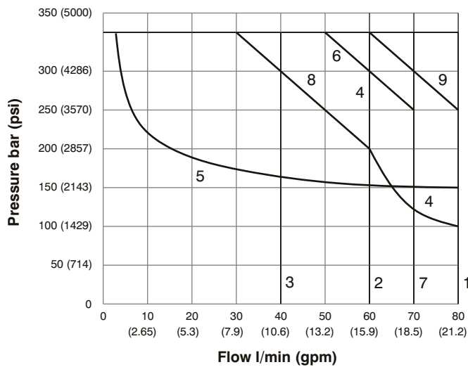
Valve with Standard AC-solenoid
