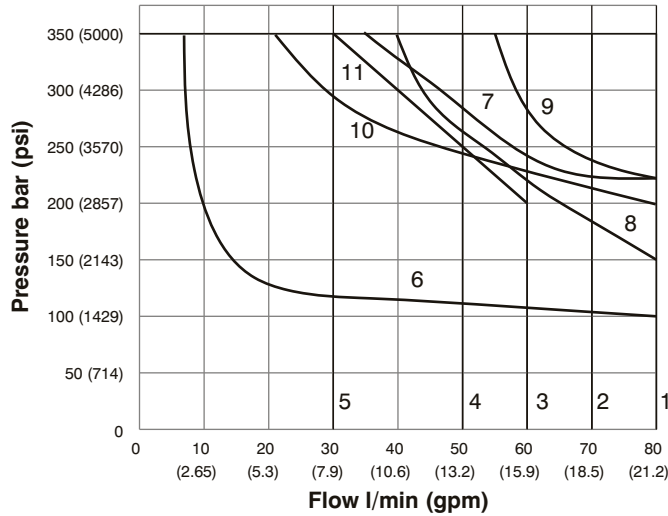
Valve with Standard DC-solenoid
